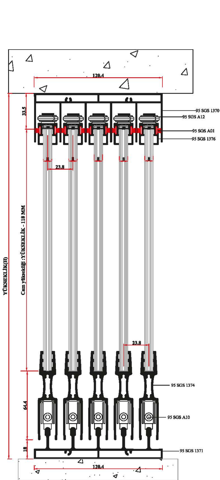
1 NOLU DETAY
