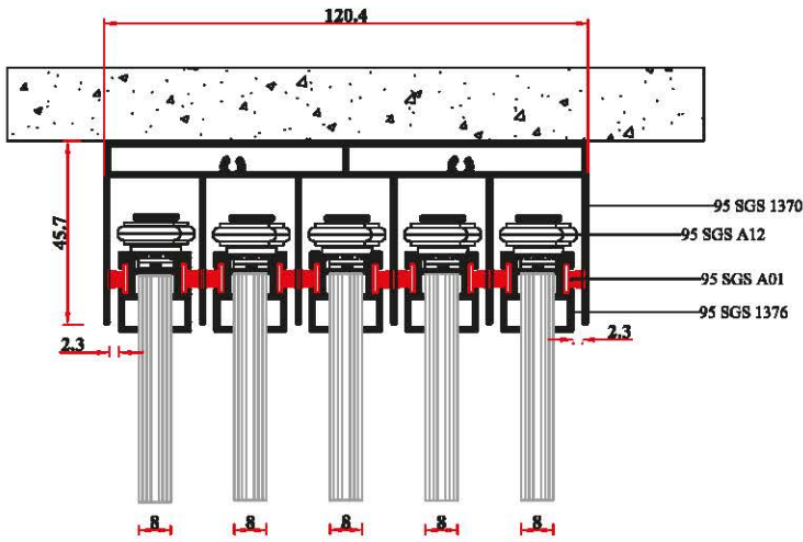
1 NOLU DETAY
