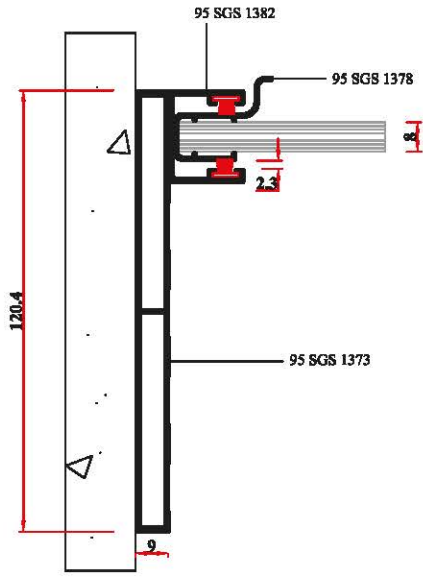
1 NOLU DETAY
